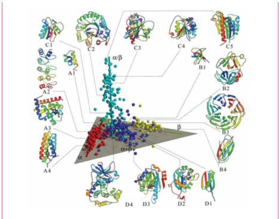
Dimensions of the Protein Universe. Protein structures are displayed here along axes signifying secondary protein structure elements: strictly \alpha helices or \beta sheets, both \alpha and \beta , or combinations of \alpha and \beta . The more complex and highly structured proteins reside at the extreme ends of the axes. In 1992, researchers estimated the number of protein families at around 1000, but the size of the protein universe has turned out to be much larger than predicted--as exemplified by the 23rd release of the Pfam database listing over 10,000 protein families. Source: NIGMS image gallery: http://images.nigms.nih.gov/index.cfm?event=viewDetail&imageID=2367 . Courtesy of Berkeley Structural Genomics Center, PSI.
